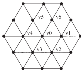
Figure 2. The subgraph B(v_0) .
