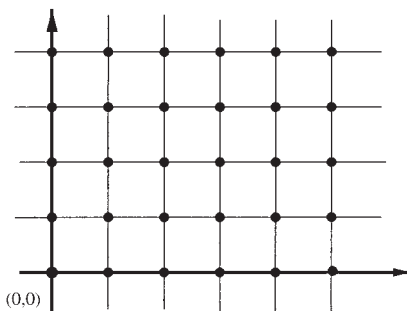
Figure 3. The square lattice \Gamma_{\square} .
