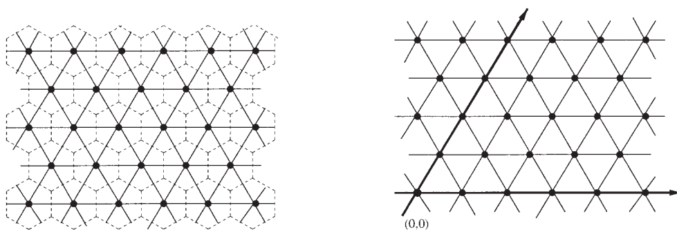
Figure 1. The hexagonal cells (left) and the triangular lattice \Gamma_{\Delta} (right).
