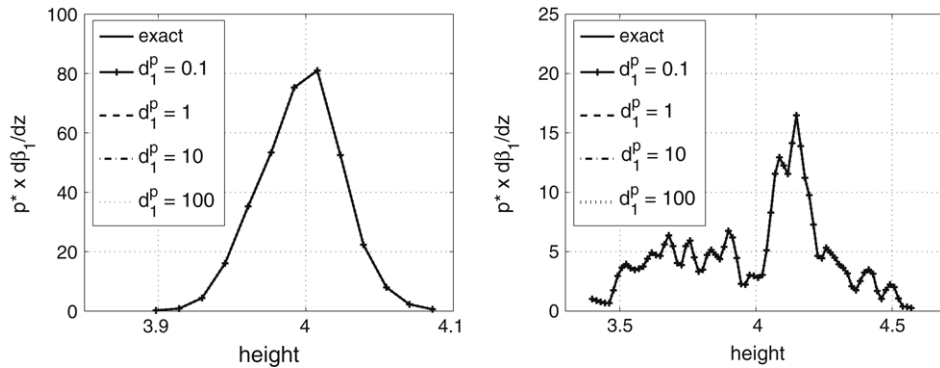
Fig. 6. The exact and the closed quantities p^* \partial b_1 / \partial z for four choices of d_k^p at t = 4 (left) and t = 9 (right). The curves are indistinguishable.
