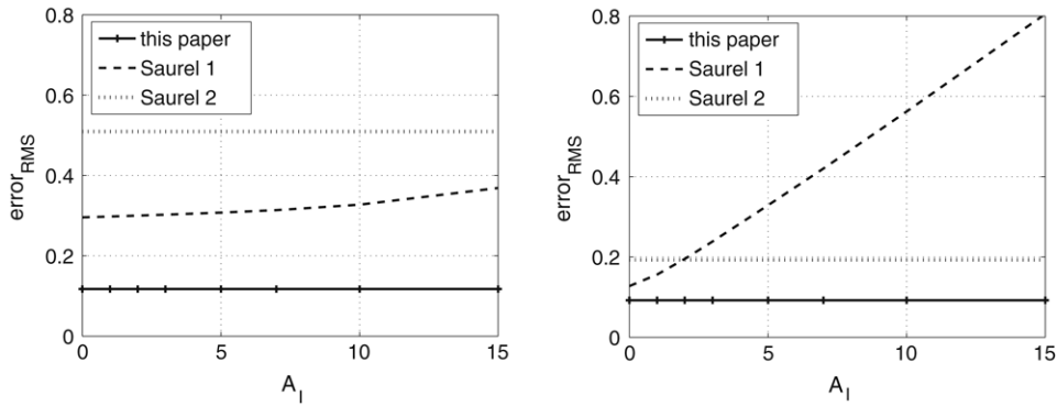
Fig. 2. Comparison of the model error (5.1) for three closures. Of these, only Saurel-1 depends on the value of A_1 as a fitting parameter; these plots serve to locate the best fit value of A_1 ( A_1 = 0 ) and thus to define the Saurel-1 closure. Left: RT, Right: RM.
