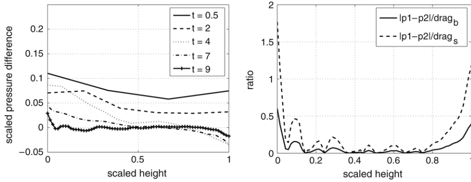
Fig. 5. Left: the scaled pressure difference \Delta \tilde{p} / (Z_2 - Z_1) is plotted vs. the scaled height (z - Z_1) / (Z_2 - Z_1) at t = 0.5, 2, 4, 7, 9 for the RT surface tension data. Right: the ratio of pressure difference and unit drag force \rho_k (\Delta v)^2 / (Z_2 - Z_1) at t = 9 .
