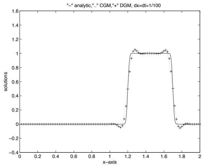
(b) \Delta x = \Delta t = \frac{1}{100}
