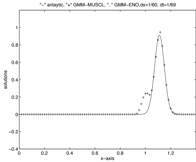
(a) \Delta x = \frac{1}{60}, \Delta t = \frac{1}{69}
