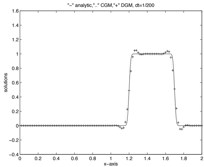
(c) \Delta x = \frac{1}{100}, \Delta t = \frac{1}{200}
