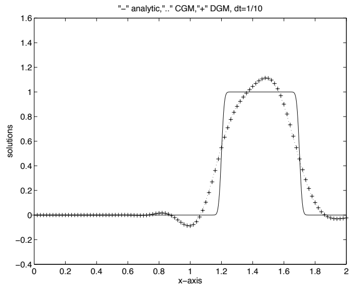
(a) \Delta x = \frac{1}{100}, \Delta t = \frac{1}{10}
