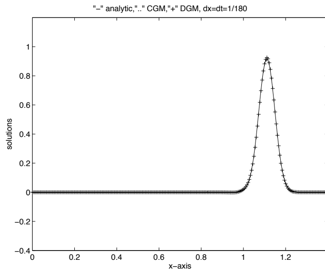
Fig I.4 Continuous and discontinuous Galerkin methods
